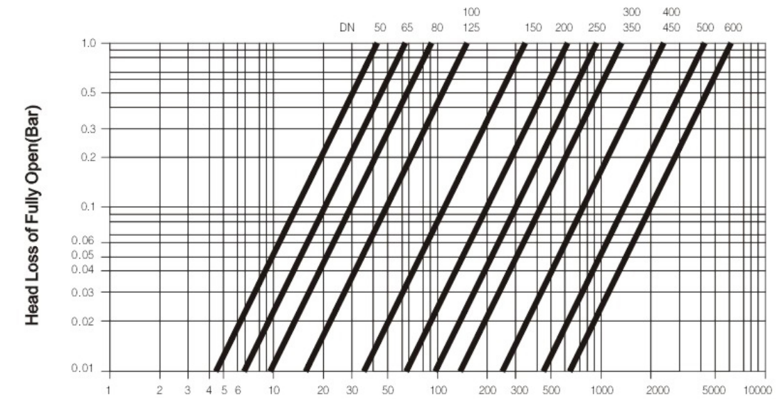
Flow chart of fully opened main valve
