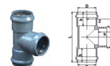
Three Faucet Regular Tee
